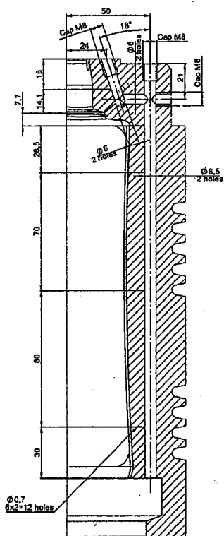
SECTION B-B
